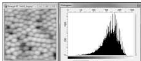
Figure 3. Histogram of the nano-surface image.
