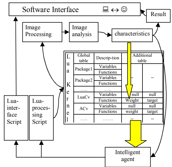
Fig. 3. Script generation cycle for image processing and analysis.
